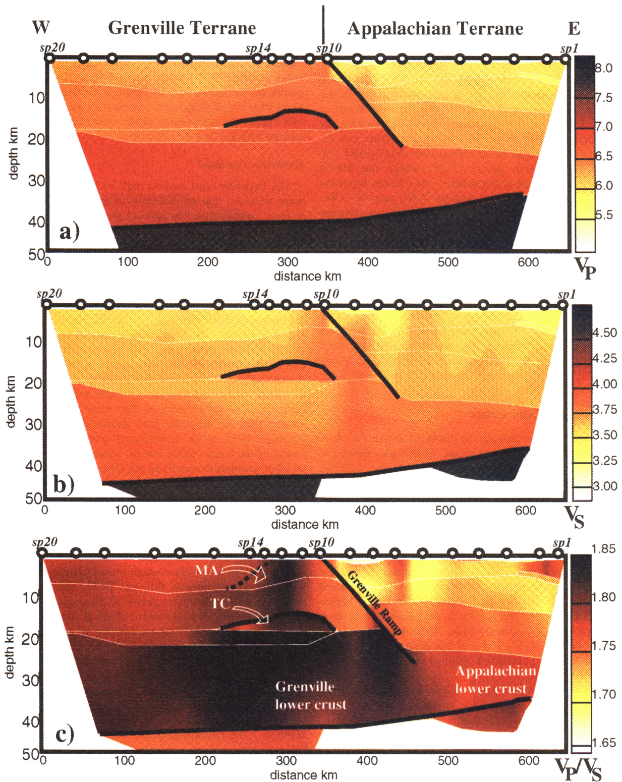
Plate 1. (a) V_P , (b) V_S , (c) V_P/V_S ratios. The combined P and S wave modeling clearly show that the difference in seismic properties between the Grenville and Appalachian Provinces can be followed at depth down to the Moho. The highest V_P/V_S ratios are found in the Grenville Province and are associated with P wave velocities in the range of 6.6–7.0 km/s. M. A., Marcy Anorthosite; T. C., Tahawus Complex.
