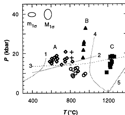
Fig. 5. Equilibration pressure-temperature determinations on Sierra Nevada xenoliths (19, 21). Trends A, B, and C are explained in the text. Symbols: ○, feldspathic granulites; ◇, garnet clinopyroxene rocks; ▲, garnet peridotites and garnet websterites; +, spinel peridotites from the CS; ■, spinel peridotites from the HS. Curves: 1, present-day geotherm in the central Sierra Nevada (22); 2, the garnet breakdown reaction: pyrope + grossular = anorthite + 2 diopside + spinel; 3, spinel-garnet peridotite transition; 4, wet peridotite solidus; 5, dry peridotite solidus (23). m_{1\sigma} , 1\sigma minimum error for the data set; M_{1\sigma} , 1\sigma maximum error for the data set.
