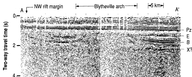
and X, crystalline basement. The depth of reflections (in kilometers) is about three times the travel time in seconds below Pz plus the amount of time above Pz.
